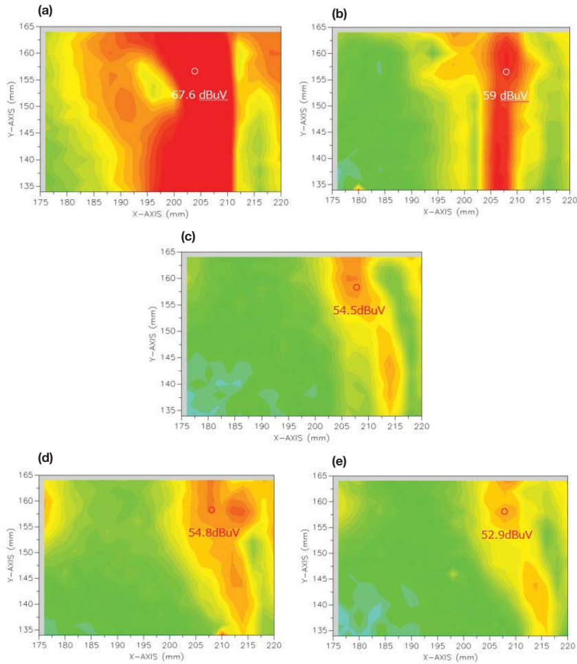
5. Measured E-field level results are given for solutions with no shield (a), an existing shield (b), ferrite and copper (c), permalloy with no ground (d), and permalloy with ground (e).
