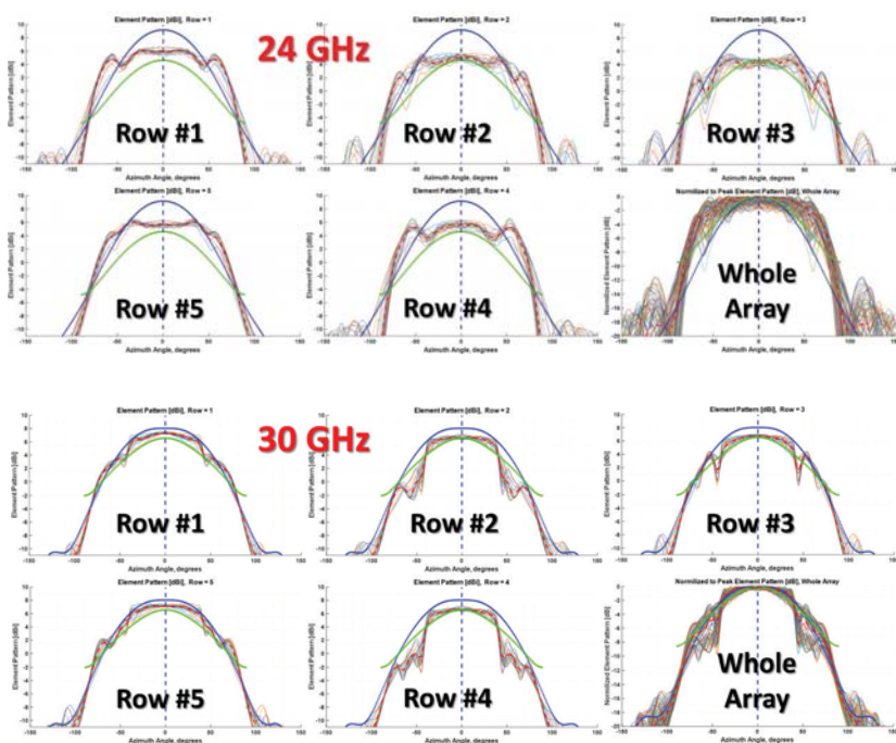
1. Shown are the active patterns of the 5- \times -16 array in rectangular lattice at 24 GHz (top) and 30 GHz (bottom).
